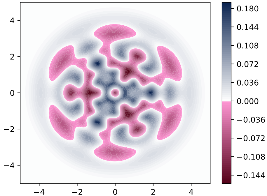
Wigner Colormap
