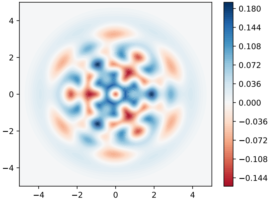
Standard Colormap
